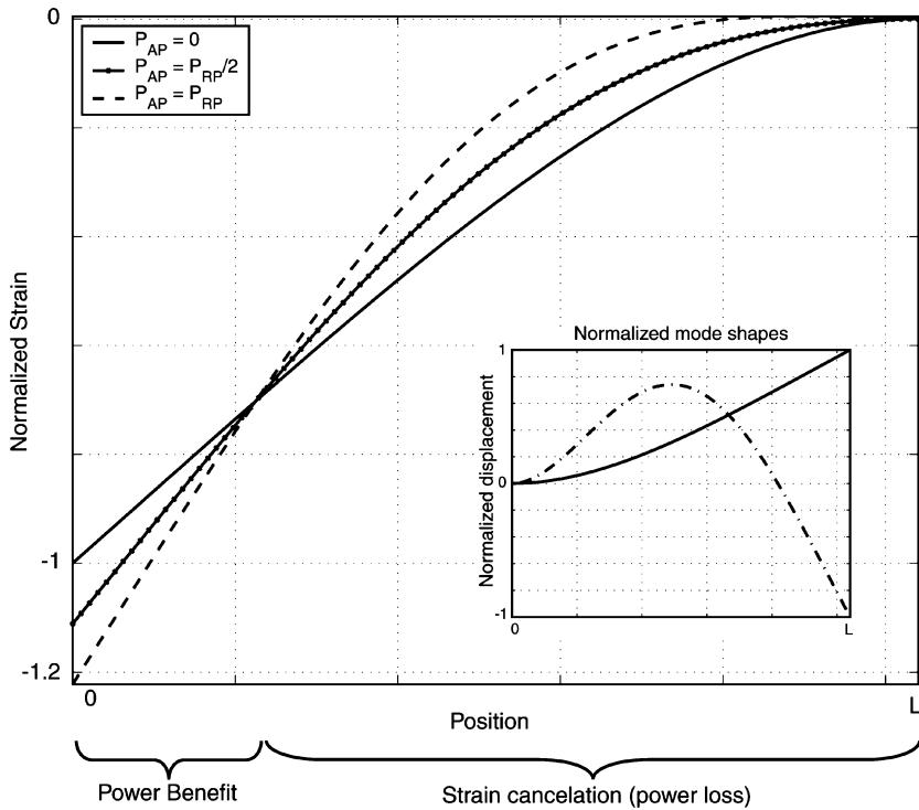
Figure 6. Strain distribution for a beam excited by multiple input vibration components, illustrating net power loss.
